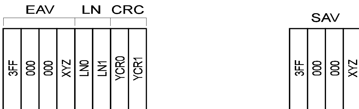
Figure 2 – Timing reference format (luminance channel shown)
