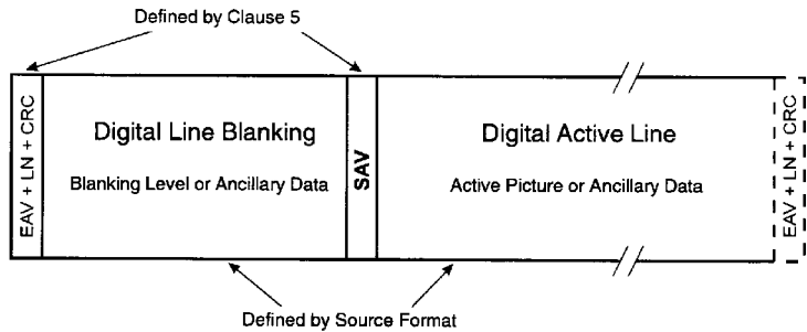
Figure 1 – Television horizontal line data
